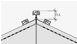
FLA = First-Latten-Abstand
